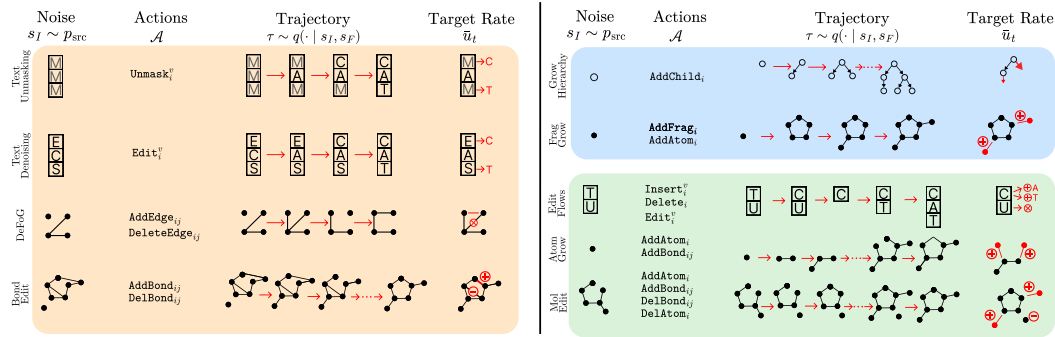
Figure 6: Examples of different existing methods that can be seen as instances of Trajectory Matching (text unmasking, text denoising, DeFog GraphGeneration Qin et al., 2025 and EditFlows Havasi et al., 2025 ) and our new instantiations of Trajectory Matching (AtomGrow, FragGrow, MolEdit, BondEdit, and GrowHierarchy). for each instantiation, we show an initial state s_I \sim p_{src} , the action space \mathcal{A} , a sample trajectory \tau from s_I to a final state s_F \sim p_{tgt} and the Rao-Blackwellized target rate \bar{u}_t(s, a | s_I, s_F) of an intermediate state s .
