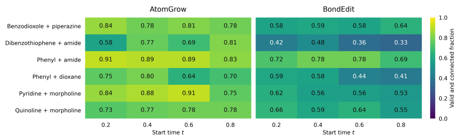
Figure 12: Substructure linking on six seed pairs (rows) and four Euler start times (columns), reporting the valid-and-connected fraction of generated molecules. ATOMGROW (left) sets s_I to the union of both seeds and uses both as roots of the action DAG; BONDEDIT (right) is adapted by sampling a target size, freezing both seeds, and requiring inserted bonds to link them. ATOMGROW substantially outperforms the factorized baseline across all pairs and start times.
