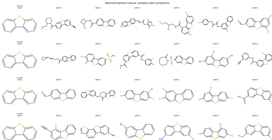
(a) Dibenzothiophene seed (out-of-distribution: not present in ZINC).
