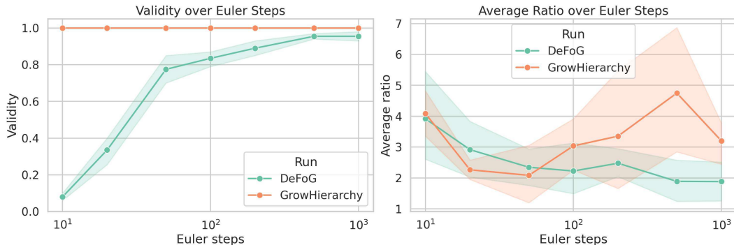
Figure 7: Validity (left) and Ratio (right) on the Tree benchmark as a function of the number of Euler integration steps. GROWHIERARCHY preserves 100% validity across three orders of magnitude of step budgets, while DeFoG’s validity collapses below \sim 10\% at 10 steps. Average Ratio metric is comparable for both.
