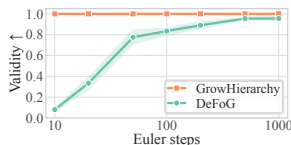
Figure 3: Tree validity by sampling steps.
