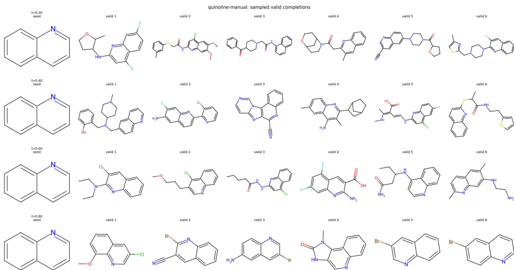
(b) Quinoline seed.
