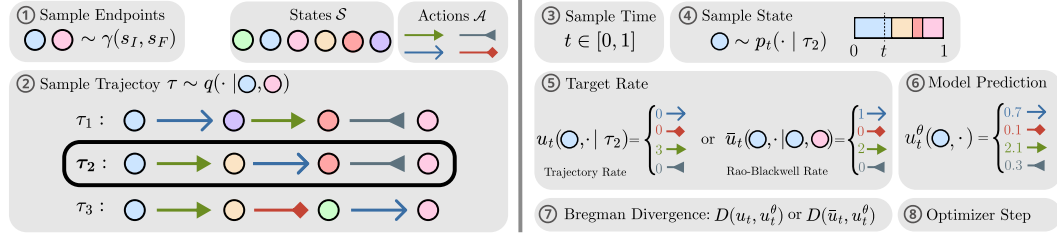
Figure 1: Training step of trajectory matching. Conditioning on a full trajectory (rather than endpoints alone) yields tractable training targets for general action spaces (including multi-component, dependent, or size-changing actions). Pseudocode in Algorithm 1.
