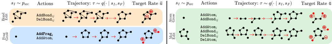
Figure 2: Four trajectory-matching instantiations on molecular graphs, BONDEDIT (factorized bond edits), FRAGGROW (fragment-based growth), ATOMGROW (atom/bond growth from a seed), and MOLEDT (noisy-initial editing), each shown with a sampled source s_I , action set, example trajectory \tau , and Rao-Blackwellized target rate \bar{u}_t . Full definitions in App. E, more instantiations in Fig. 6
