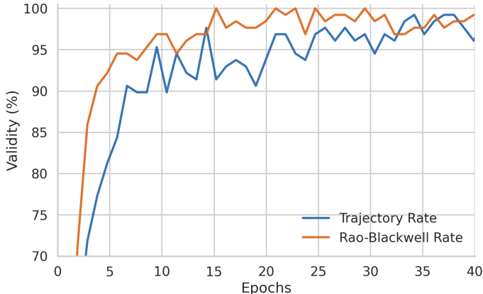
Figure 9: Training dynamics on ZINC under ATOMGROW: the Rao-Blackwellized target \bar{u}_t converges faster and with lower epoch-to-epoch variance than the trajectory-conditioned target u_t , while reaching the same final validity. The behavior matches the variance-reduction guarantee of Prop. B.3.
